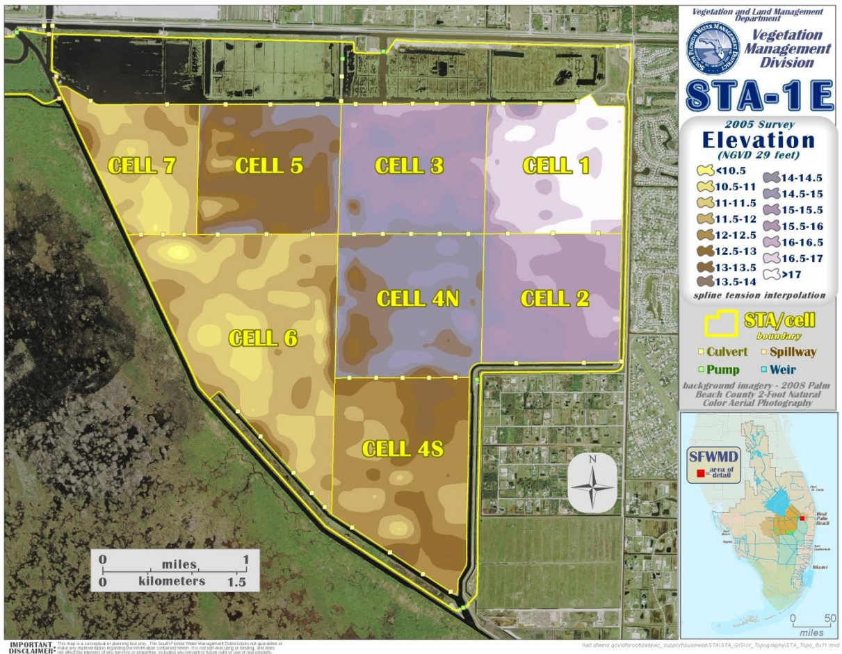
Figure 6. STA-1E DEM based on 2005 Topographic Survey Data
