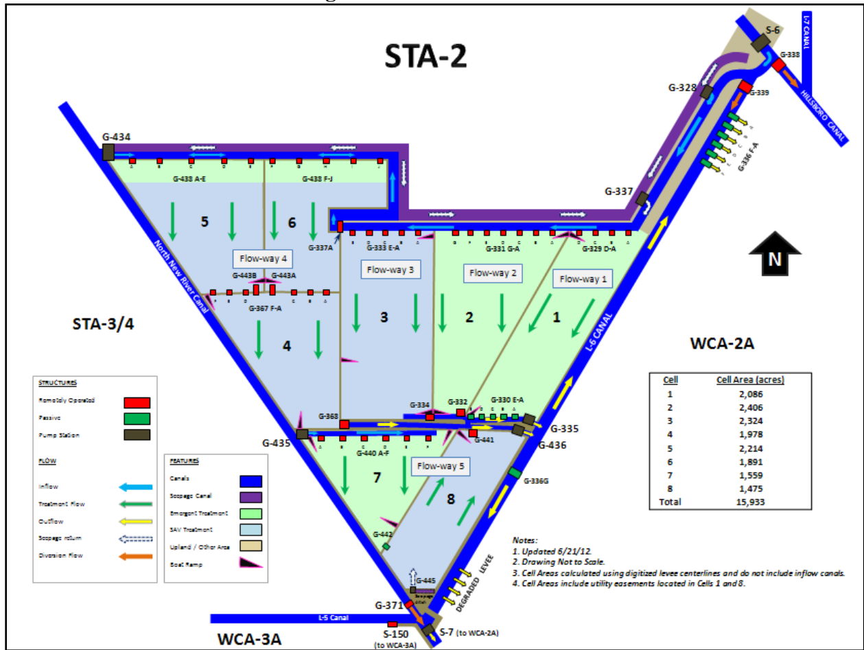
Figure 3. STA-2 Schematic
