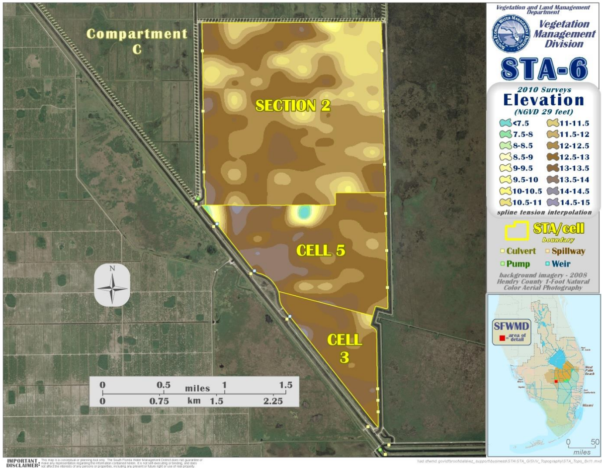
Figure 11. STA-6 DEM based on 2010 Topographic Survey Data
