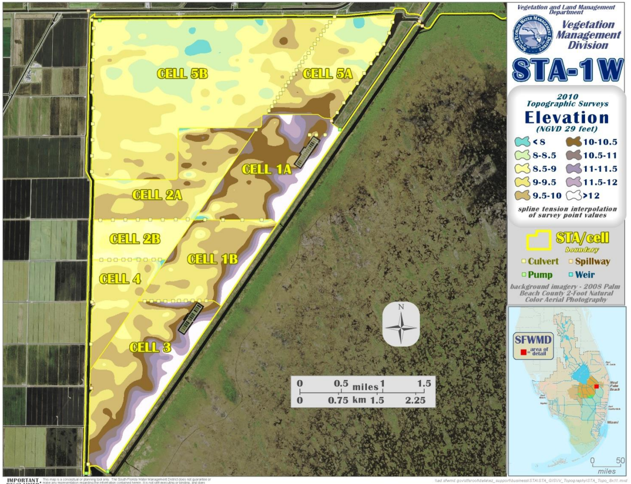
Figure 7. STA-1W DEM based on 2010 Topographic Survey Data
