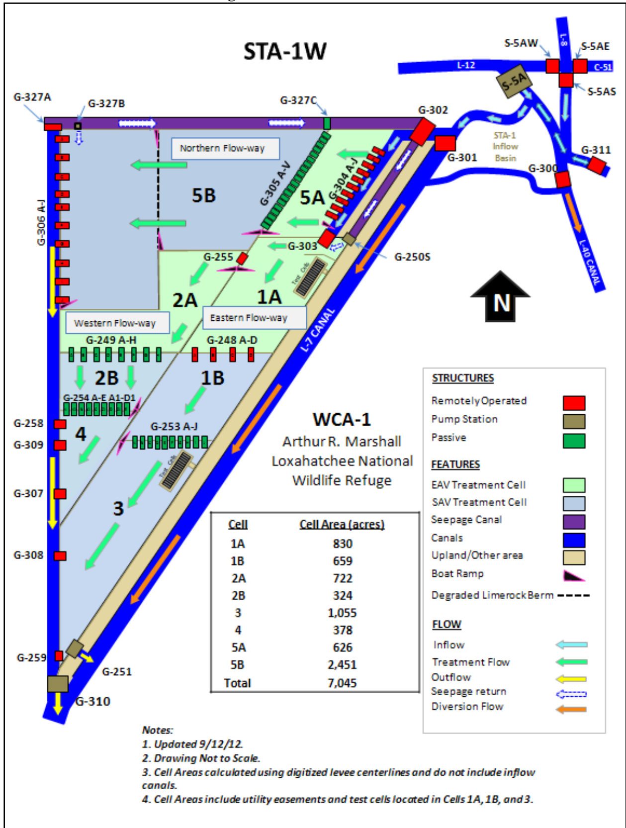
Figure 2. STA-1W Schematic
