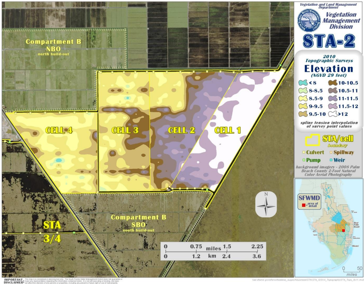
Figure 8. STA-2 DEM based on 2010 Topographic Survey Data
