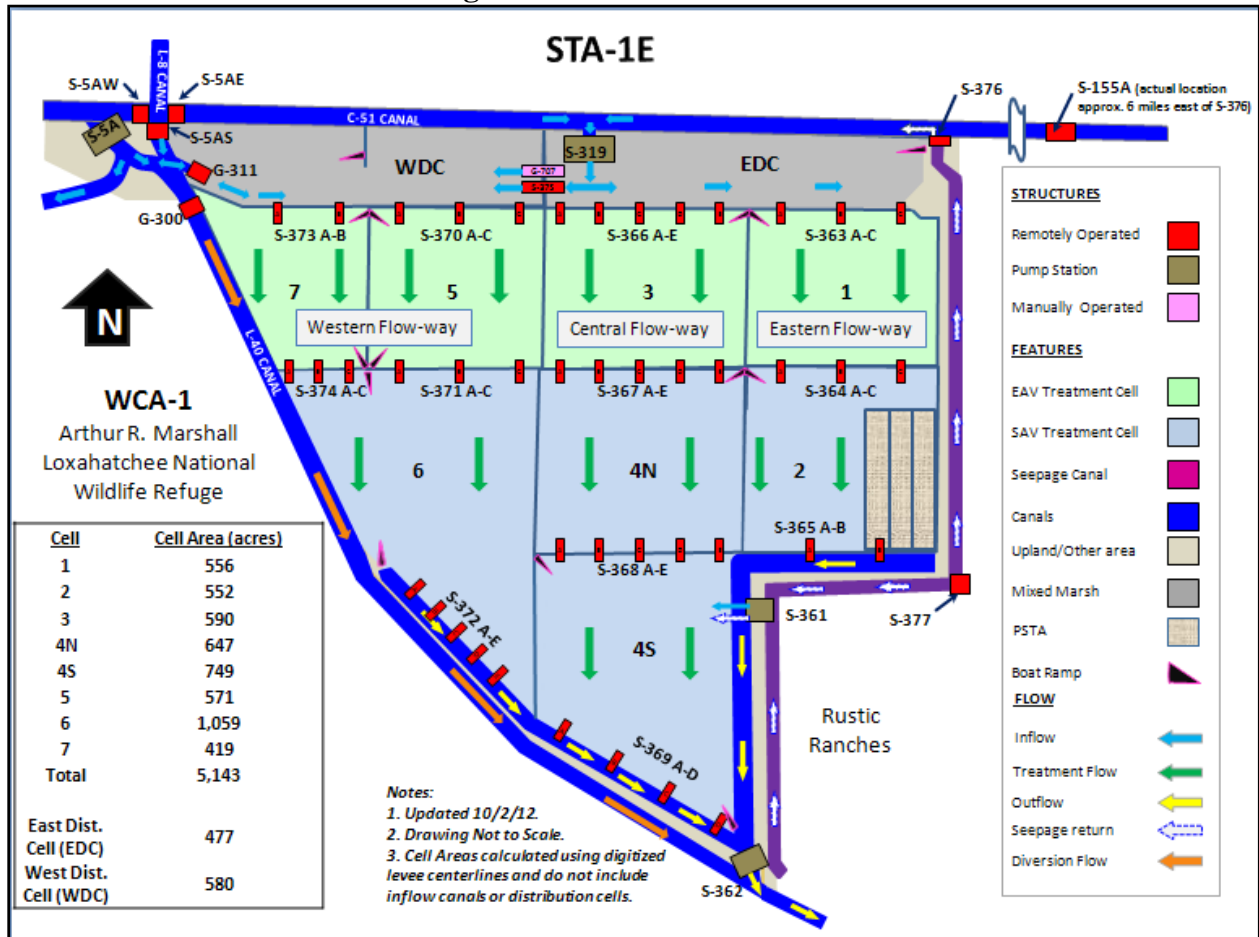
Figure 1. STA-1E Schematic
