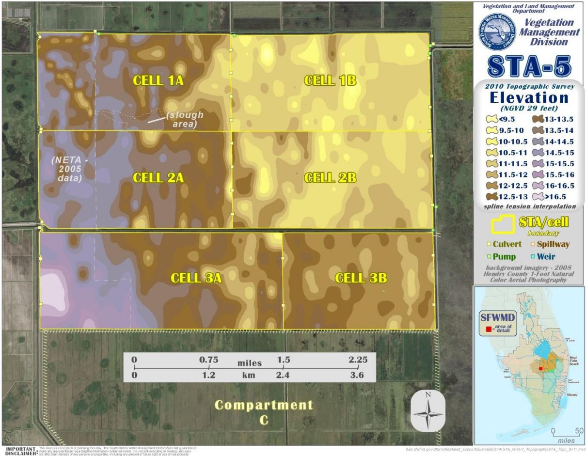
Figure 10. STA-5 DEM based on 2010 Topographic Survey Data
