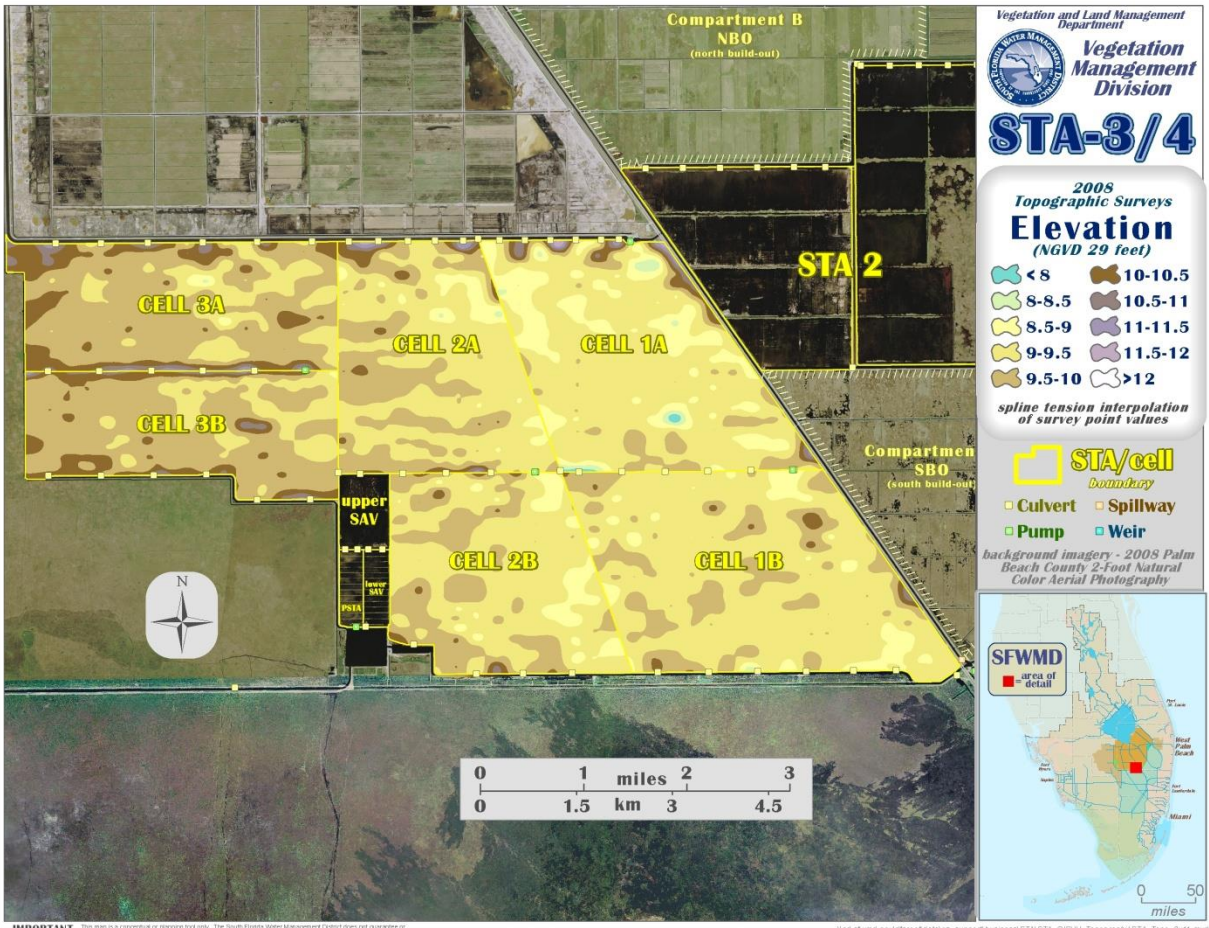
Figure 9. STA-3/4 DEM based on 2008 Topographic Survey Data
