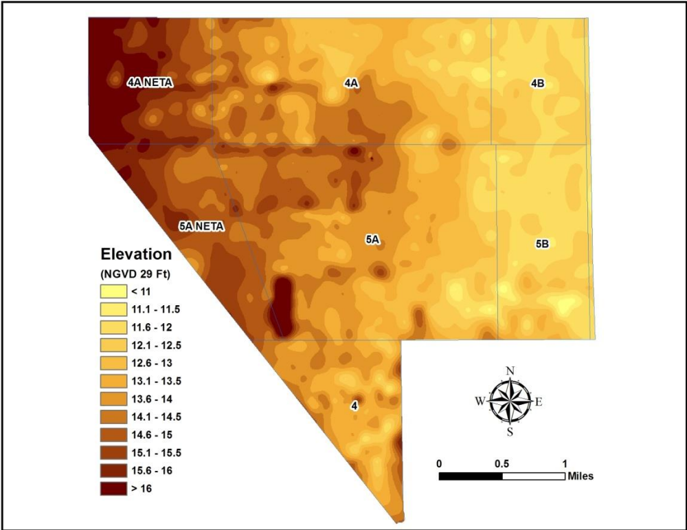
Figure 13. Compartment C* DEM based on 2006 Topographic Survey Data (*The Compartment C treatment cells are now referred to as STA-5 Cells 4A, 4B, 5A, 5B and STA-6 Cell 4).
