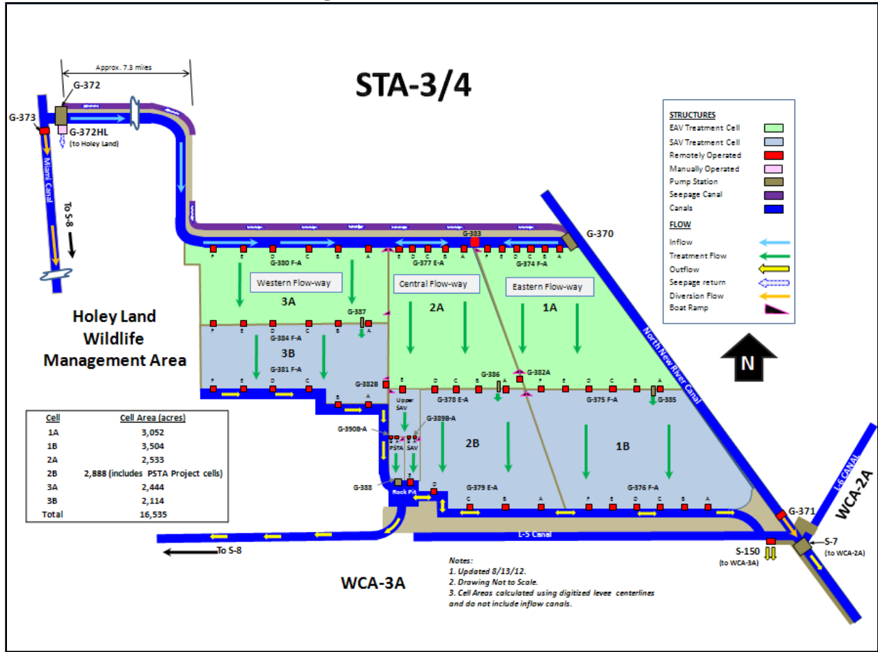
Figure 4. STA-3/4 Schematic
