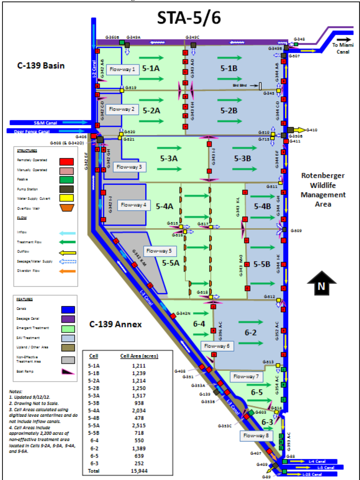
Figure 5. STA-5/6 Schematic
