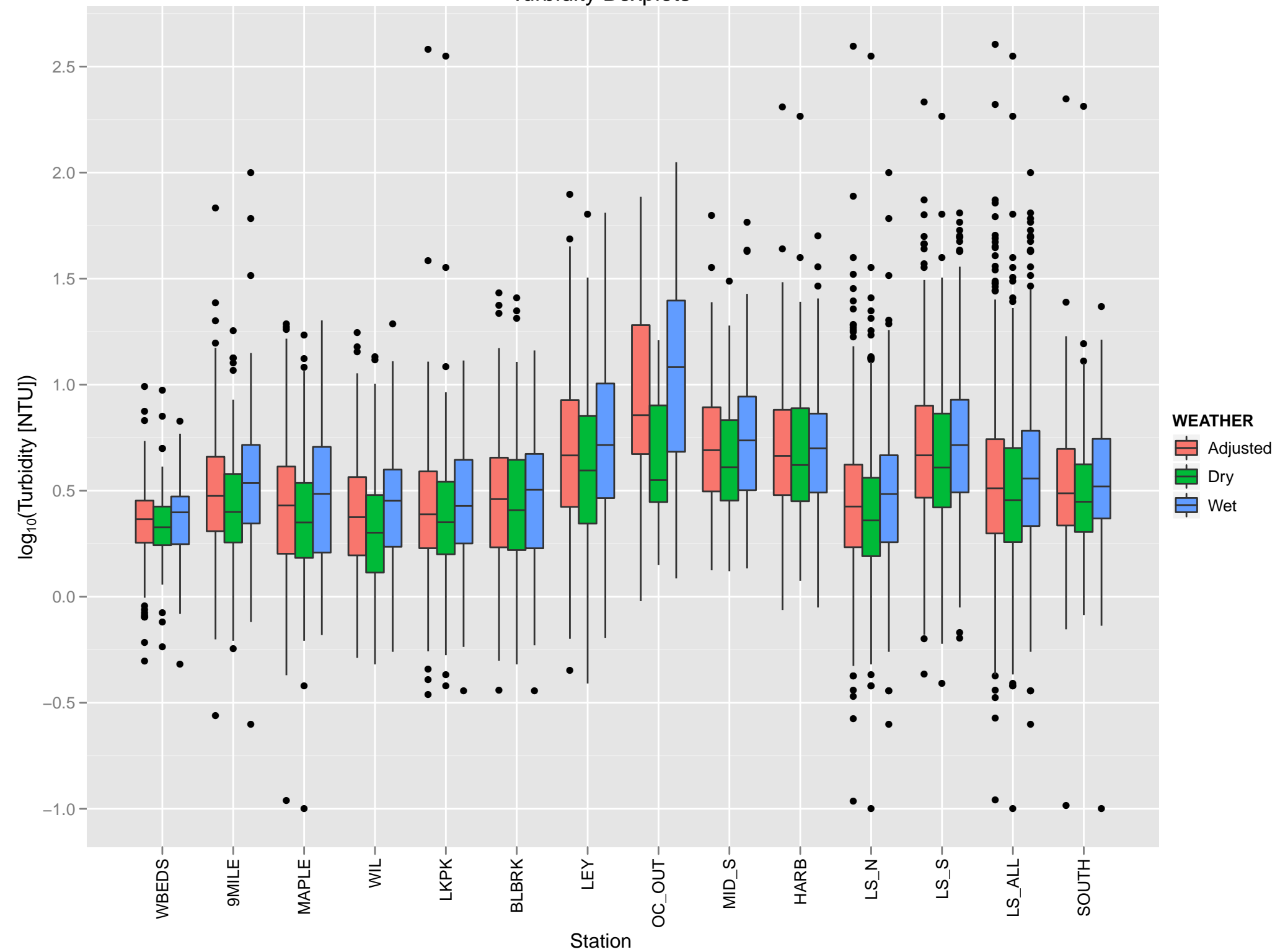
Turbidity Boxplots
